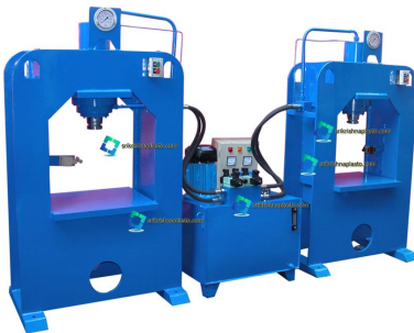
Double Station Hydraulic Tile Press Paver Block Making Machine
