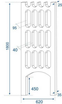
RCC Tree Guard Making Mould FDTG180035-25
