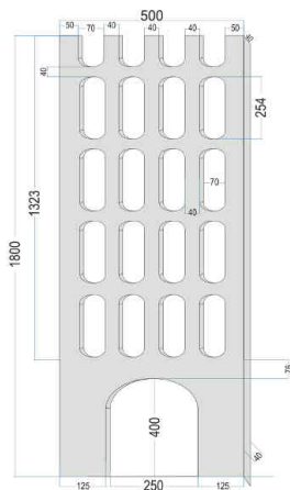
Tree Guard Mould FDHTG
