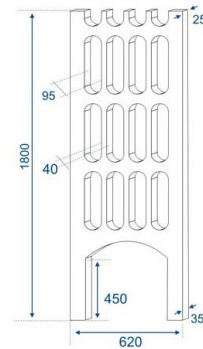
RCC Tree Guard Making Mould FDTG180035-25
