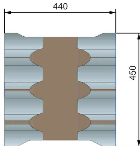
Saucer Drain Cover Mould 450mm X 440mm X 100mm
