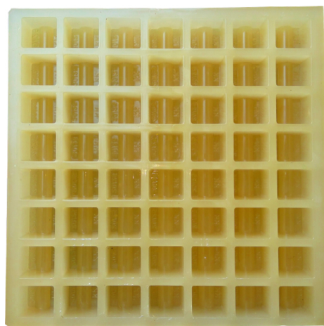
20mm - 25mm Concrete Cover Block Rubber Mould
